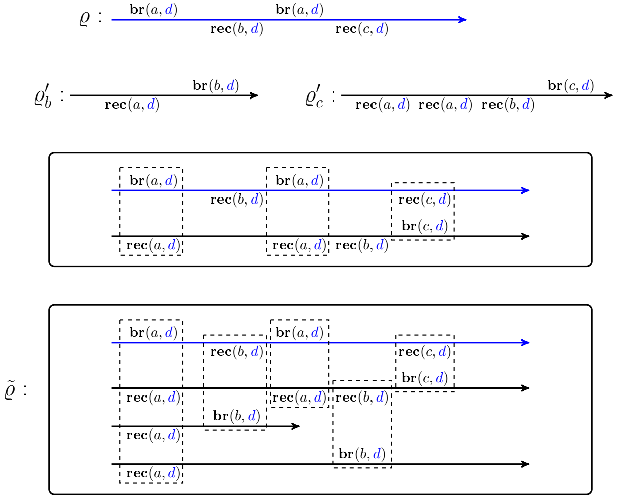
Figure 3.8: An illustration of the proof of Lemma 3.35. The partial run \rho is compatible with decomposition (a, b, a, c, \varepsilon) . We have \mathbf{In}_d(\rho_b) = a \in \mathcal{L}_{(a)} and \mathbf{In}_d(\rho_b) = aab \in \mathcal{L}_{(a,b,a)} . We build \tilde{\rho} such that \mathbf{In}_d(\tilde{\rho}) = \varepsilon . We start by using \rho'_c to eliminate the unmatched receptions of c (while adding some unmatched receptions of b ), then we use \rho'_b to eliminate the unmatched receptions of b . We ignore data other than d in this picture.
